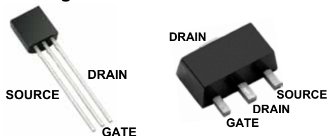
TO-92
